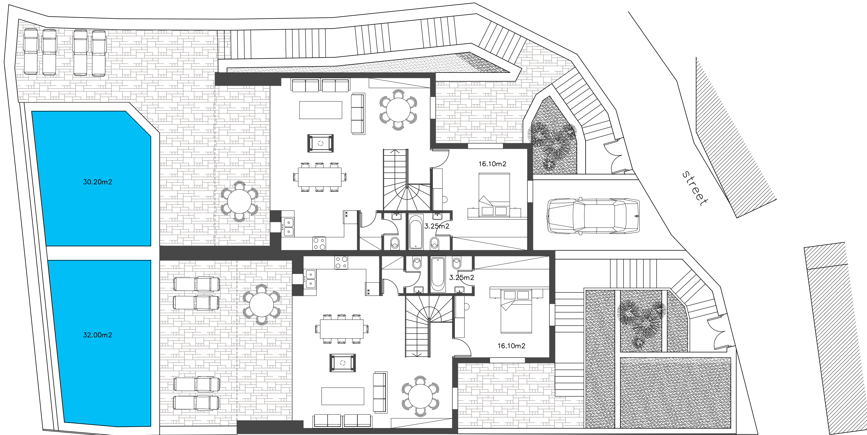
1st floor 1:100
