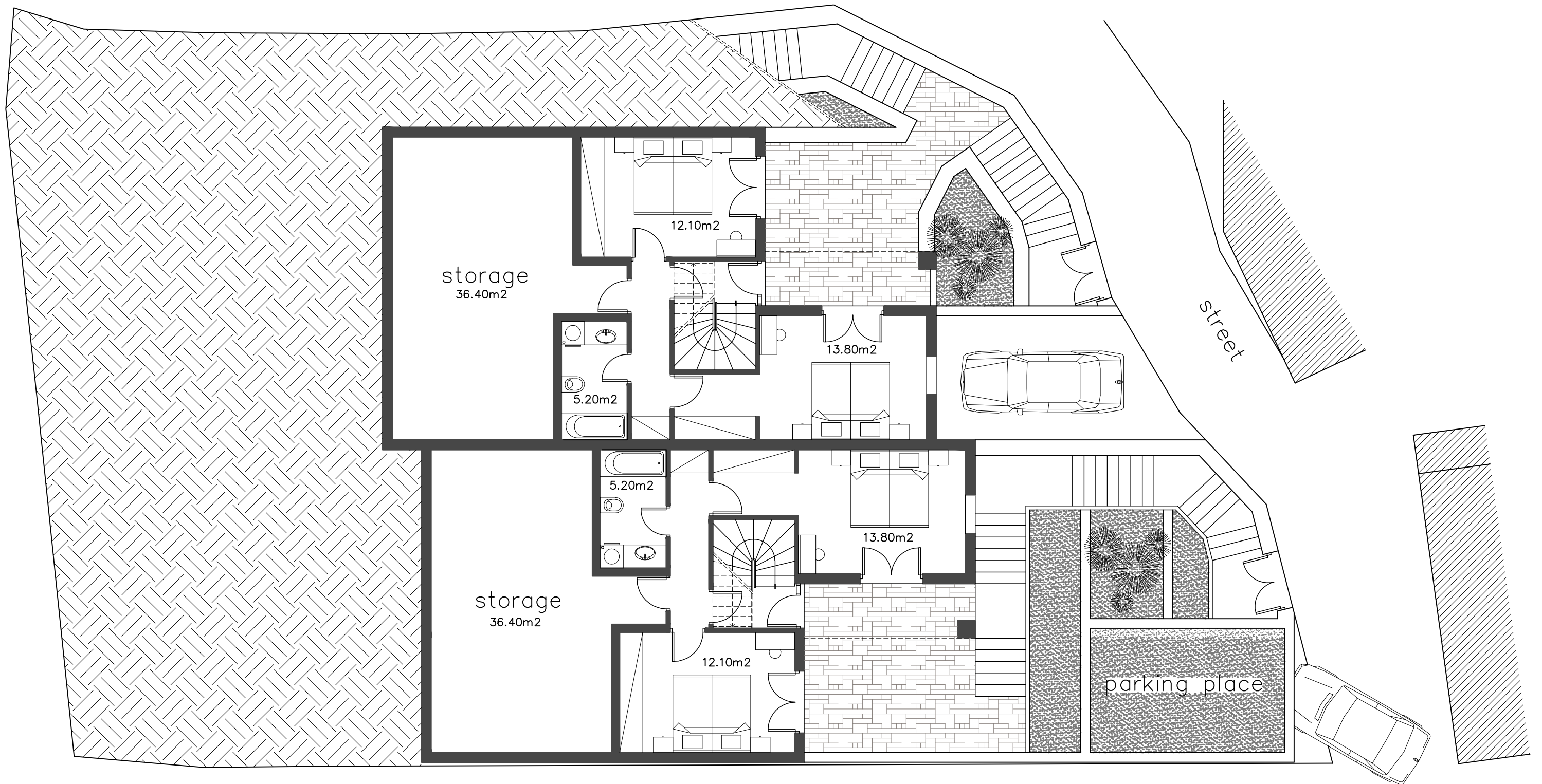
ground floor 1:100
